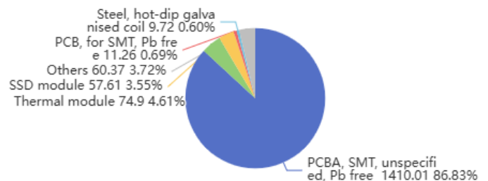
Figure 2. Hotspot Analysis of Raw Material [Emission Factor]
